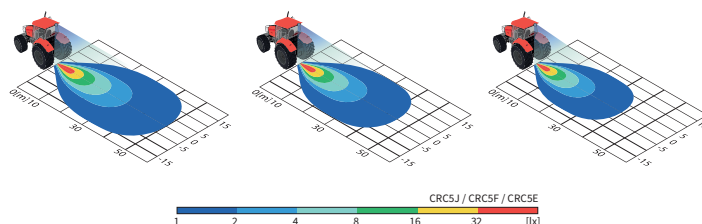
Lamp positioning: 8° from the vertical plane, h=2,5m
